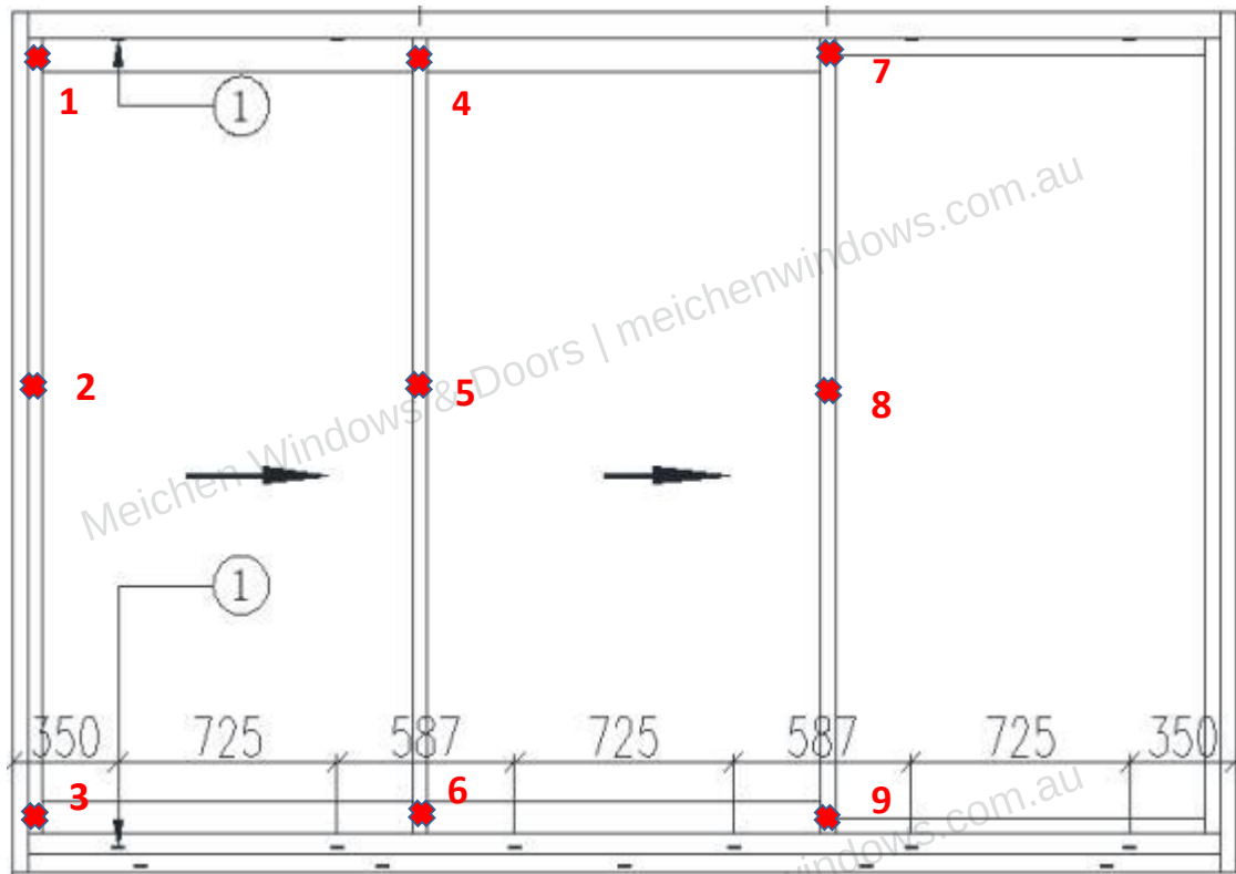
Fig. 1.1 Locations of Displacement Measuring Devices
