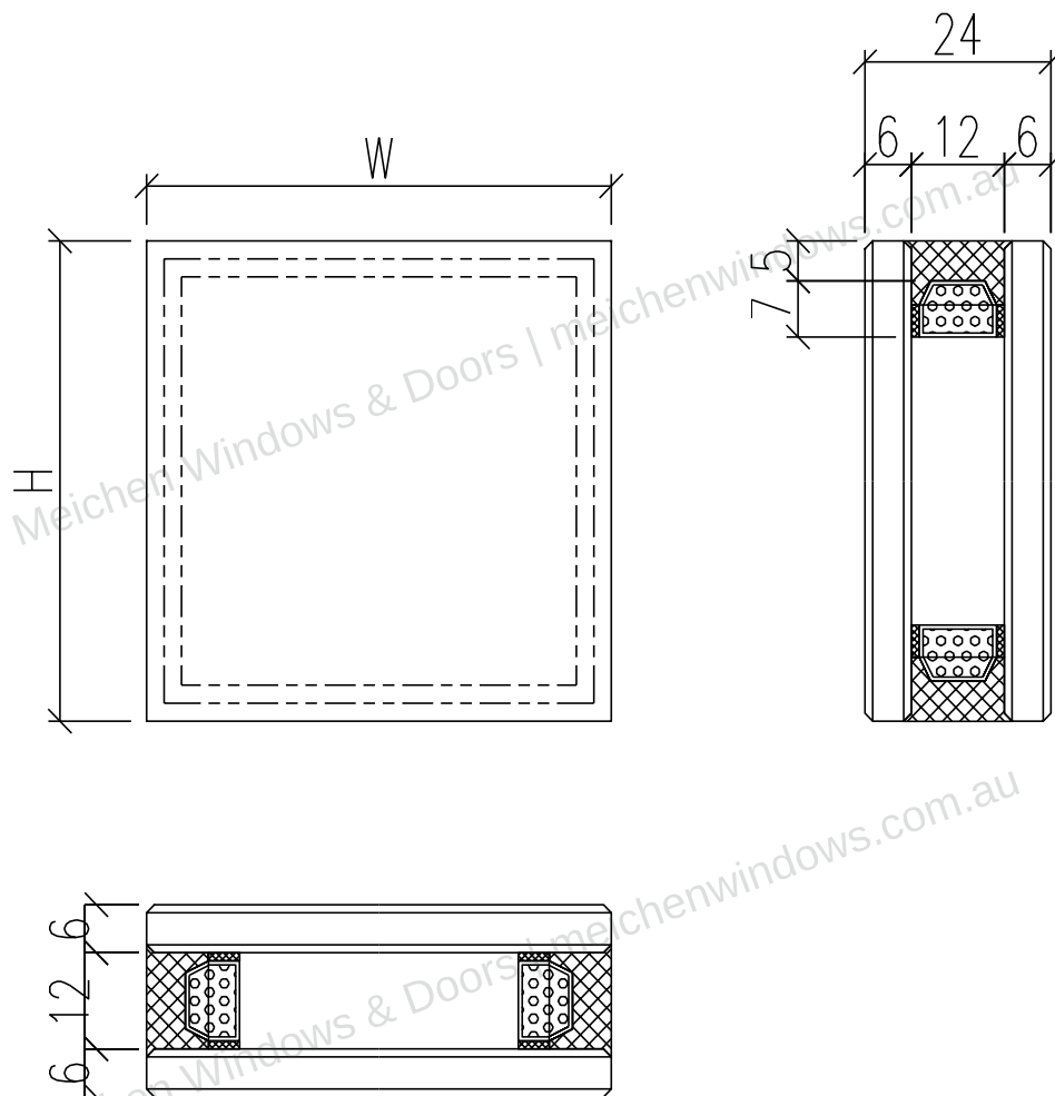
Fig. 9 Drawing of glazing
